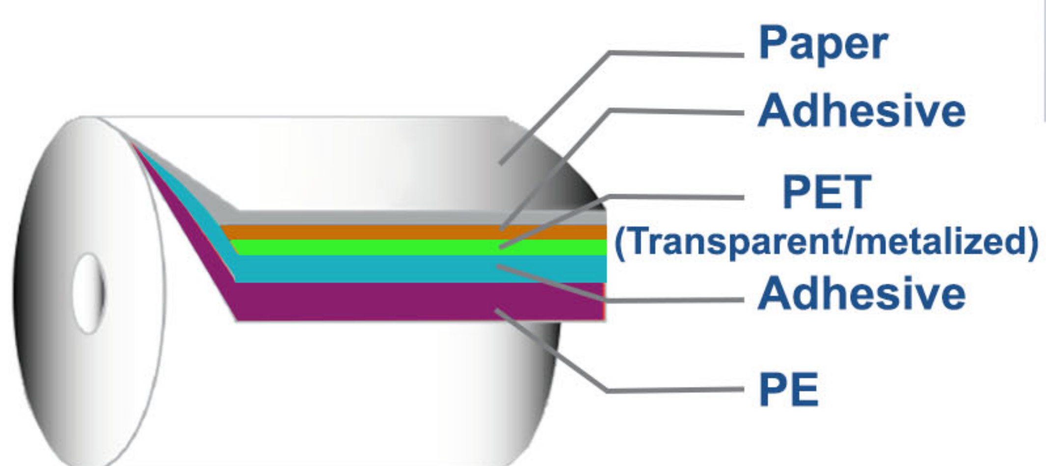
Three Layer Film with Paper
